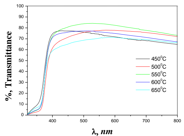
Fig. 2. Optical transmittance spectra of ZnO films doped with Al atoms and thermally treated at different temperatures.
